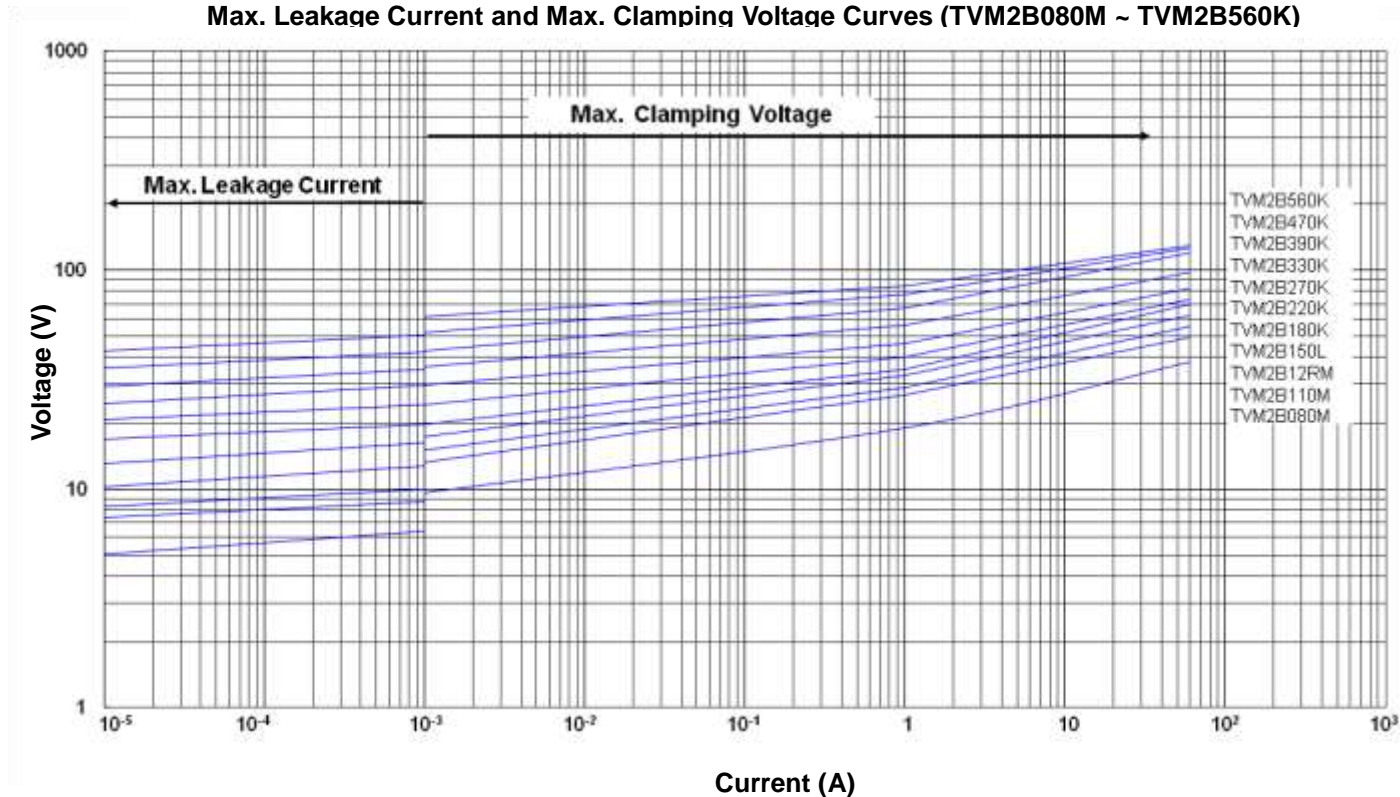
Max. Leakage Current and Max. Clamping Voltage Curves (TVM2B080M ~ TVM2B560K)
