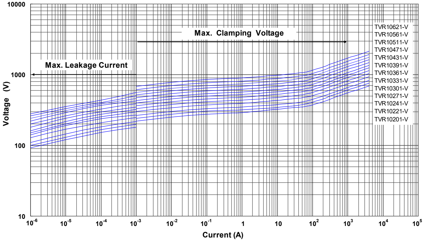
Max. Leakage Current and Max. Clamping Voltage Curves (TVR10201-V to TVR10621-V)
