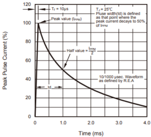
Fig.3 - Pulse Waveform
